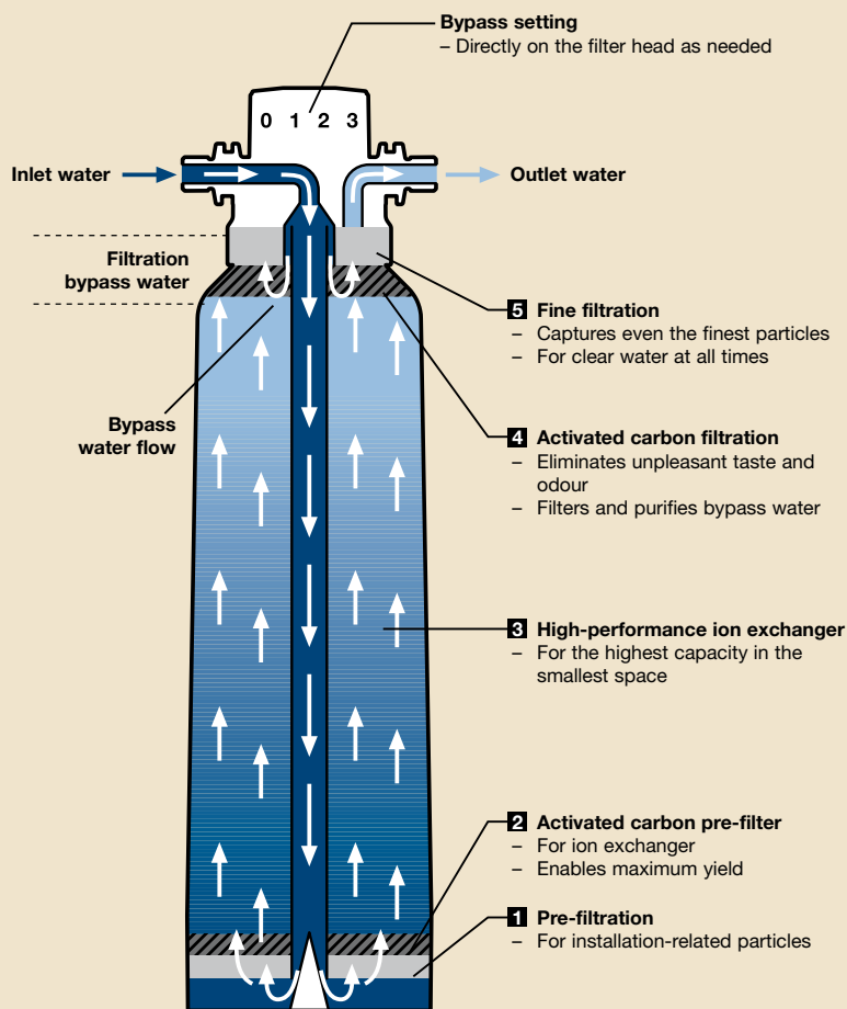
Configuration of a BWT bestmax PREMIUM filter cartridge with 5-way filtration
